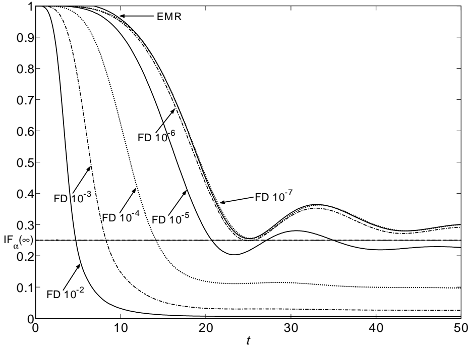
Figure 1: IF_\alpha(t) by finite differences (FD) for \varepsilon = 10^{-i} with i \in \{2, \dots, 7\} and by the present method (EMR).
