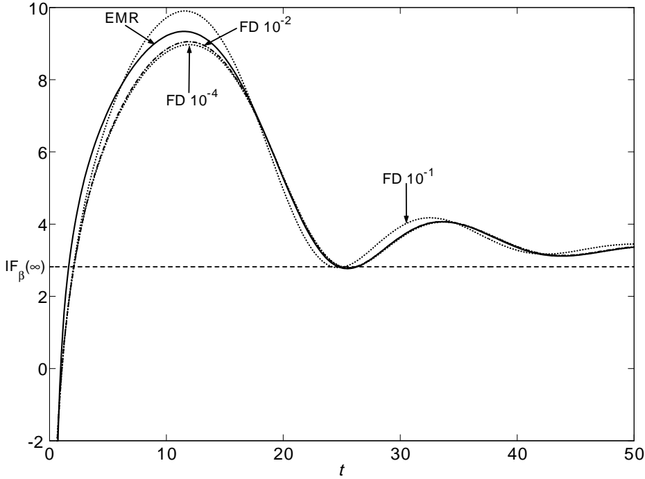
Figure 2: IF_\beta(t) by finite differences (FD) for \varepsilon = 10^{-i} with i \in \{1, 2, 4\} and by the present method (EMR).
